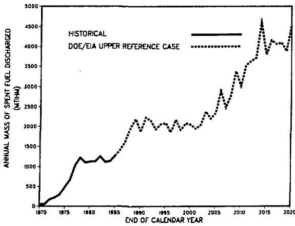
Fig. 5. Projected Mass (MTIHM) of Annual Commercial Spent Fuel Discharges for the DOE/EIA Upper Reference Case.
