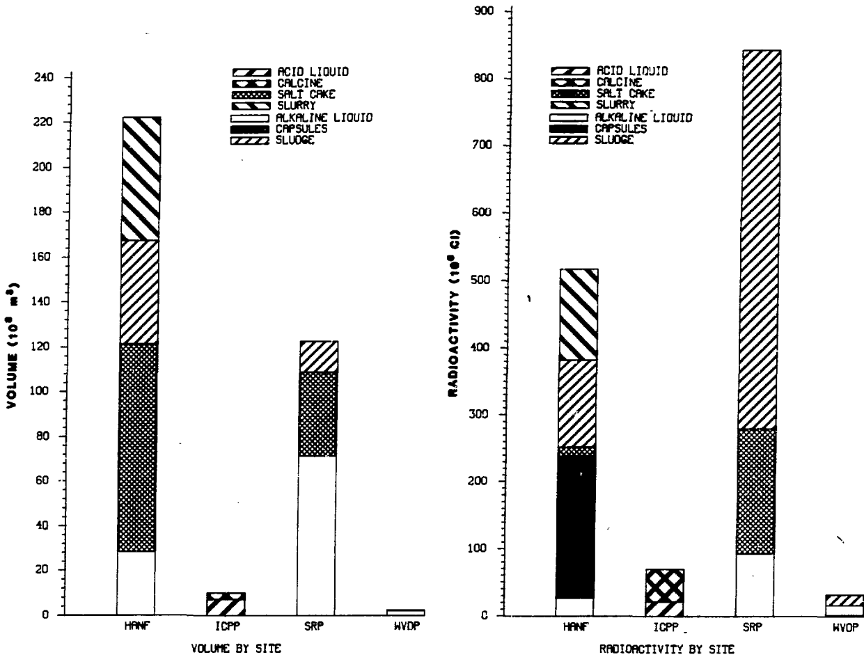
Fig. 7. Distribution of Volume and Radioactivity of HLW by Site and Type Through 1985.
