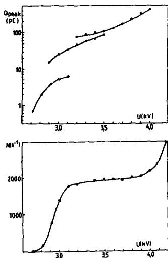
Fig. 2. The charge (up) and counting (down) characteristics of streamer tube in absence of a magnetic field.
