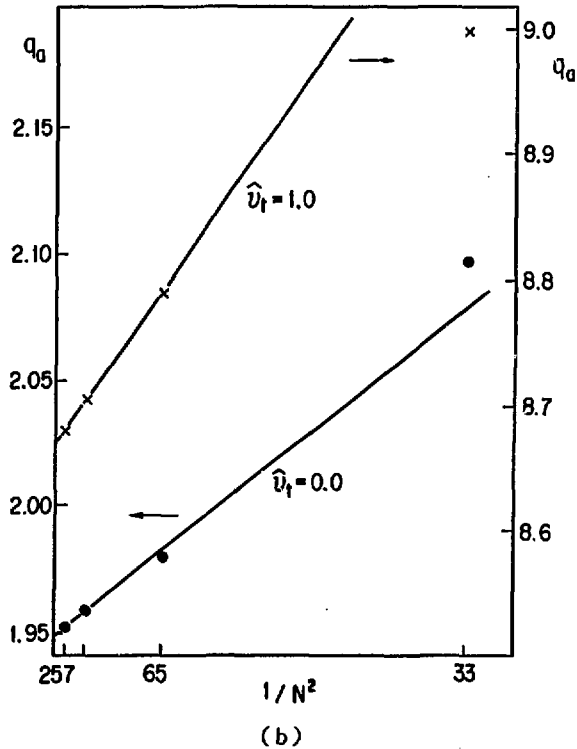
Fig.1 Convergence study: The dependence of relevant parameters on the mesh size is displayed, i.e the number of radial grid points N=NR=2NZ is indicated. a) The poloidal flux on axis \psi_0 for zero and unity flow on axis \hat{u}_1=0 and 1. b) The safety factor on surface q_a for zero and unity flow on axis \hat{u}_1=0 and 1. c) The position of the magnetic axis for zero and unity flow on axis \hat{u}_1=0 and 1.
