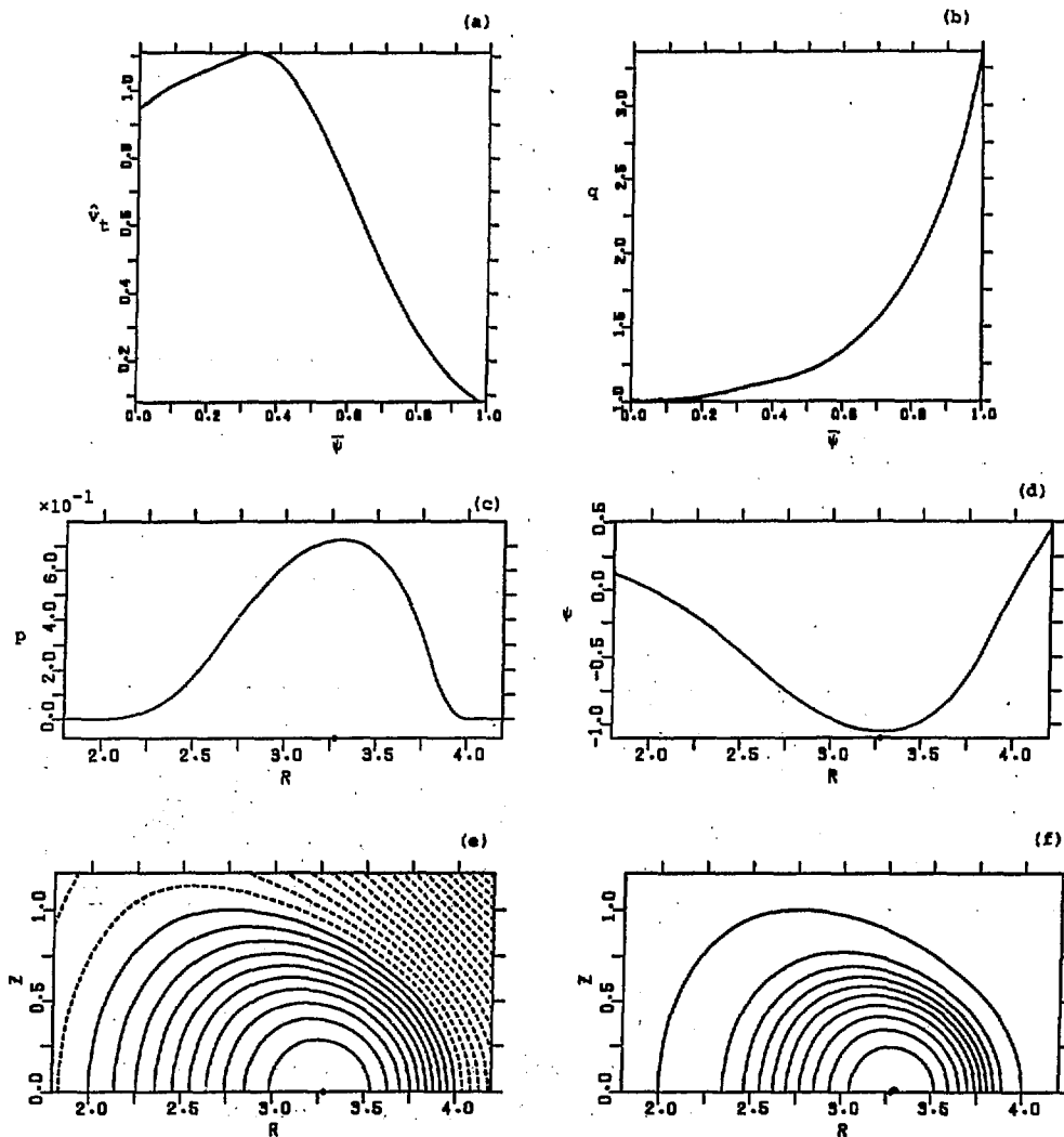
Fig.7 Equilibrium with toroidal flow. The p_0(\bar{\psi}) and F(\bar{\psi}) profiles are the same as for Fig.6; the flow has to multiplied by the factor 0.5 (Fig.7(a)). The safety factor q is a smooth function (Fig.7(b)). The total pressure p=p(r, z=0) (Fig.7(c)) and the poloidal flux \psi=\psi(r, z=0) (Fig.7(d)) are displayed as functions of r in the midplane z=0 . The contour lines of constant flux (Fig.7(e)) and pressure (Fig.7(f)) do not coincide.
