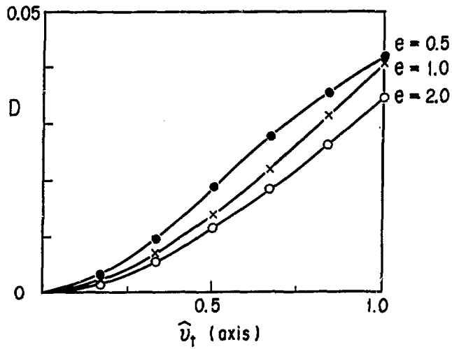
Fig.2 Shift of the magnetic axis D=R_e(\theta)/R_e(0)-1 with increasing flow velocity.
