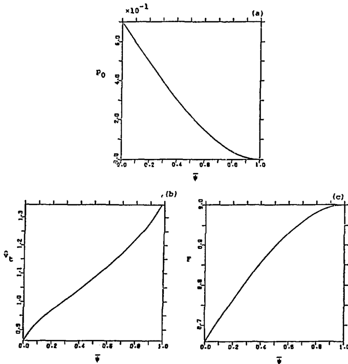
Fig.5. Equilibrium with toroidal flow. The pressure function p_0(\bar{\psi}) has to be reduced by the factor 0.7 (Fig.5(a)) and the flow \hat{v}_t(\bar{\psi}) by 2/3 (Fig.5(b)); the toroidal field F(\bar{\psi}) is unchanged (Fig.5(c)). The safety factor q has a dip (Fig.5(d)). The total pressure p=p(r, z=0) (Fig.5(e)) and the poloidal flux \psi=\psi(r, z=0) (Fig.5(f)) are displayed as functions of r in the midplane z=0 . The contour lines of constant flux and pressure do not coincide.
