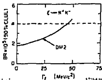
Figure 18. Upper limits from the DM2 collaboration [28] for J/\psi \rightarrow \gamma\xi(K^+K^-) as a function of the width of the \xi . The dotted line is the measured value for this branching ratio from the Mark III. Only for \Gamma_\xi \gtrsim 50 MeV/c 2 are the two experiments consistent.
