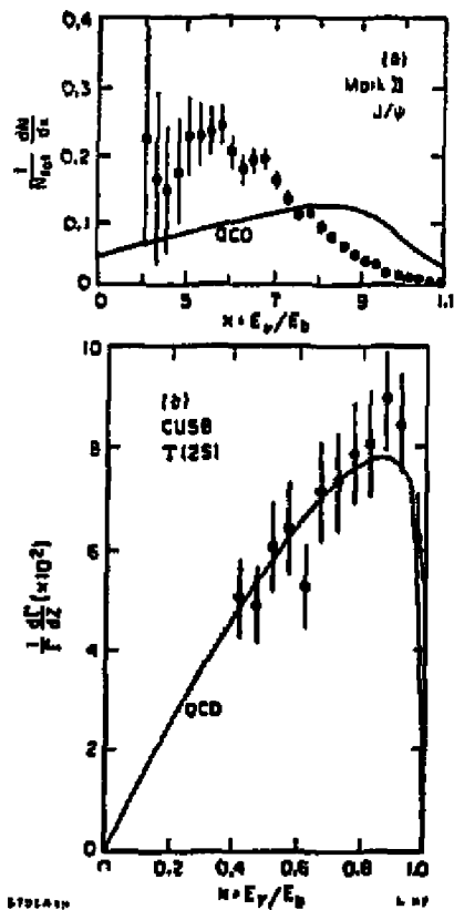
Figure 2. Comparison of data and theory with experimental resolution folded in for the process, a) J/\psi \rightarrow \gamma + X , Mark II data [9] b) T \rightarrow \gamma + X , CUSB data [10] .
