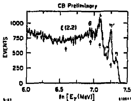
Figure 5. Preliminary crystal ball collaboration data for the process J/\psi \rightarrow \gamma + X , emphasizing the resonance region.
