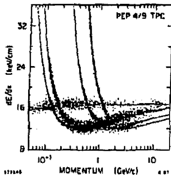
Figure 8. dE/dx spectra from the TPC/2 \gamma collaboration [5] . The resolution is \sigma/(dE/dx) = 3.6\% .
