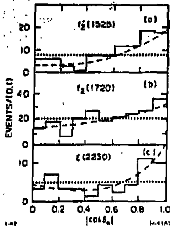
Figure 18. Mark III \cos \theta_K distributions for the events in the region: a) 1420-1550 \text{MeV}/c^2 , (b) 1620-1820 \text{MeV}/c^2 , and (c) 2180-2280 \text{MeV}/c^2 . The histograms are the data; the dotted lines are the Monte Carlo predictions for the spin 0 and the dashed lines for the spin 2 hypotheses.
