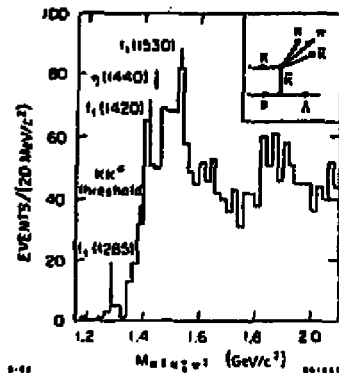
Figure 7. LASS [4] K_s K^\pm \pi^\mp invariant mass spectrum from 11 \text{ GeV}/c^2 K^- p \rightarrow K_s K^\pm \pi^\mp \Lambda .
