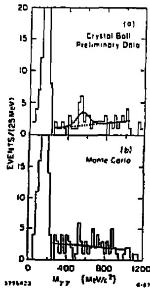
Figure 22. Preliminary Crystal Ball results for the process T \rightarrow 3\gamma after all cuts and projected to the M_{\gamma\gamma} axis. Part a) is data, part b) is Monte Carlo.
