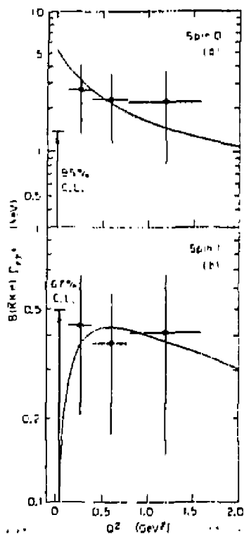
Figure 10. B(KK\pi)\Gamma_{\gamma\gamma} from the TPC/2 \gamma collaboration [3] , where the data are acceptance corrected with (a) the spin-0 Monte Carlo model and (b) spin-1 Monte Carlo model. The upper limits near q^2 = 0 come from no-tag data, where no resonance was seen. The curves are the best fits to the single-tag points of the expected (a) spin-0 and (b) spin-1 q^2 dependence.
