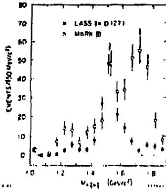
Figure 13. K_s K_s mass distributions from (open circles) Mark III uncorrected J/\psi \rightarrow \gamma K_s K_s data and (solid circles) LASS acceptance corrected K^-p \rightarrow K_s K_s A data. The LASS data have been multiplied by 0.127 to match the Mark III data in the 1525 MeV/c 2 bin. LASS used a 11 GeV/c K^- beam, and for this plot required |t'| < 2 (GeV/c) 2 , where t' = t - t_{min} .
