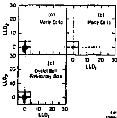
Figure 20. Log likelihood difference (LLD) for energy cluster 1 (LLD1) vs energy cluster 2 (LLD2) for the decay T \rightarrow 3\gamma . Part a) is Monte Carlo for QED 3\gamma , part b) is Monte Carlo for \gamma\eta(2\gamma) , part c) is crystal ball preliminary data.
