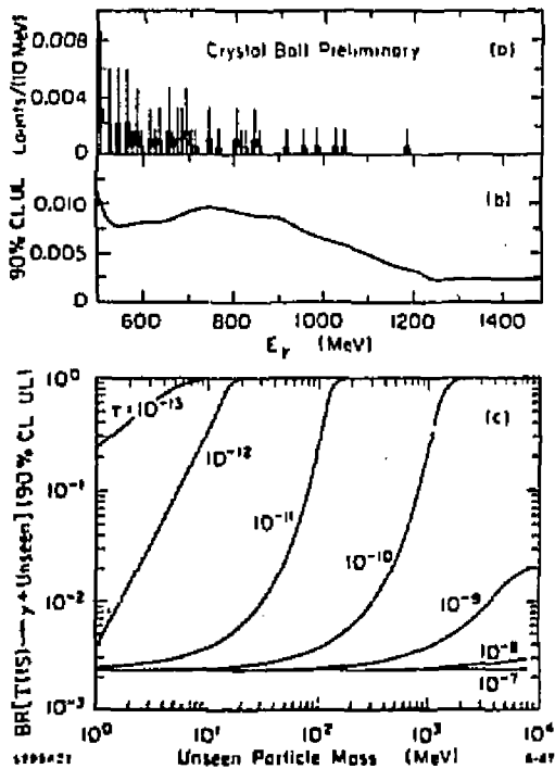
Figure 20. Preliminary results from the crystal ball for \Upsilon(2S) \rightarrow \pi\pi\Upsilon(1S) , \Upsilon(1S) \rightarrow \gamma Unseen. a) the corrected photon spectrum. b) the 90% confidence-level upper limits derived from the spectrum in a) assuming a long lived non-interacting particle. c) the limits as a function of the lifetime ( \tau ) of the unseen particle assuming that some of its decay products interact.
