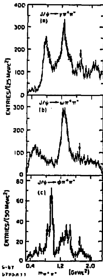
Figure 12. Mark III 21 effective mass spectra in the reactions (a) J/\psi \rightarrow \gamma \pi^+ \pi^- , (b) J/\psi \rightarrow \omega \pi^+ \pi^- , (c) J/\psi \rightarrow \phi \pi^+ \pi^- .
