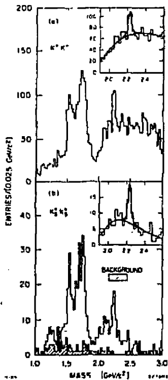
Figure 14. Mark III invariant mass distributions: Part a), K^+K^- effective mass spectrum in the radiative decay J/\psi \rightarrow \gamma K^+K^- ; part b), K_s K_s effective mass spectrum from the decay J/\psi \rightarrow \gamma K_s K_s .
