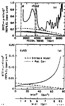
Figure 25. Limits on T(1S) \rightarrow \gamma X compared to standard model calculations for T \rightarrow \gamma Higgs. a) preliminary results from the crystal ball. The vertical dashed-dot lines show the kinematic thresholds for the relevant fermions. The horizontal dashed line corresponds to the lowest order calculation for the Wilczek mechanism. The two solid lines (roughly horizontal) indicate the range of the theoretical estimate of the first order QCD radiative corrections to the Wilczek calculation. b) similar published results from the CUSB experiment. The top solid is a smoothed experimental limit, the bottom two lines are theory as indicated in the figure.
