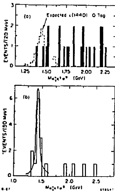
Figure 9. TPC/2 \gamma [3] , invariant K_s K^\pm \pi^\mp mass spectra from \gamma\gamma production: part a), no tag \gamma\gamma events ( q^2 \sim 0 ); the dotted histogram has the shape of an \tau signal which should have been seen if \Gamma_{\tau \rightarrow \gamma\gamma} = 1.6 keV; part b), single tag events with q^2 > 0.25 ; the solid line is a Monte Carlo calculation for the expected shape of an E(1420) meson with phase space decay.
