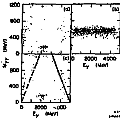
Figure 21. M_{\gamma\gamma} vs E_\gamma for the decay T \rightarrow 3\gamma after all but the final cut. Part a) is Monte Carlo for QED 3\gamma , part b) is Monte Carlo for \gamma\gamma(2\gamma) , part c) is crystal ball preliminary data. The lines on part c) represent the final cut. All data to the upper right of the solid line and upper left of the dashed line are cut. Note that part c) has two entries per event, and thus the dashed line is a reflection of the solid line.
