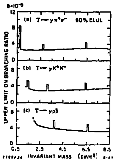
Figure 23. Results from CLEO [34] for 90% -confidence-level upper limits on branching fractions as functions of the invariant mass of the two hadrons for (a) T \rightarrow \gamma \pi^+ \pi^- , (b) T \rightarrow \gamma K^+ K^- , and (c) T \rightarrow \gamma p \bar{p} . These limits assume a particle width of less than 100 MeV/c 2 .
