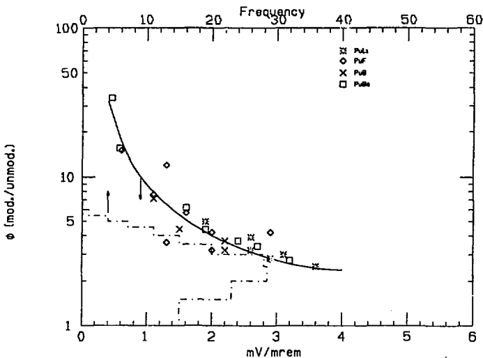
Figure 9. Sensitivity of TLD's versus mod./unmod. fluence ratios with Research Area ratios inscribed.
