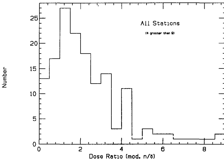
Figure 3. Frequency of fast neutron/gamma-ray dose ratios in the Research Yard.
