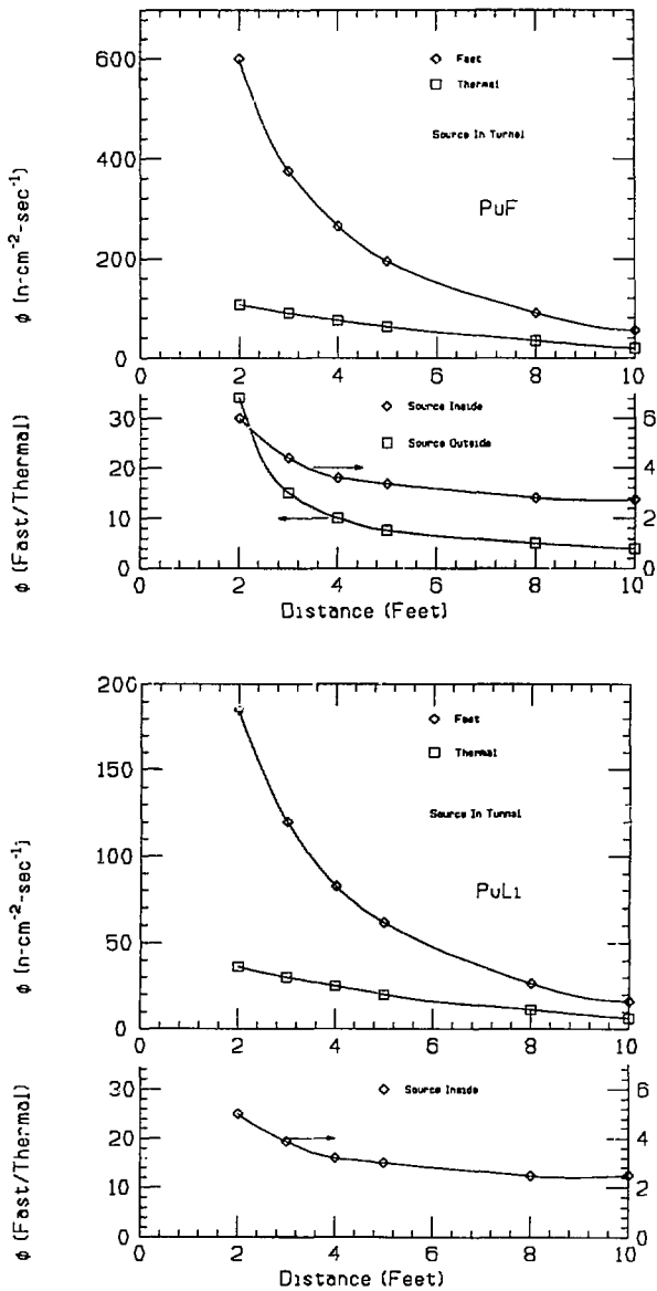
Fig. 7c-d. Mapping of Tunnel Neutrons.
