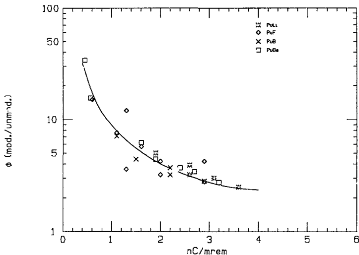
Figure 8. Sensitivity of TLD's versus mod./unmod. fluence ratios.
