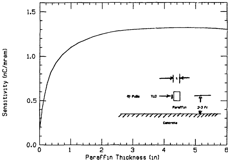
Figure 6. TLD sensitivity as a function of paraffin thickness.
