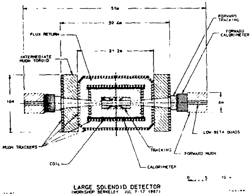
Fig. 4. Large Solenoid Detector from the Berkeley SSC Workshop.
