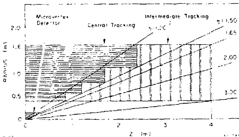
Fig. 9 Schematic view of central and intermediate tracking systems in the Large Solenoid Detector from the Berkeley SSC Workshop.
