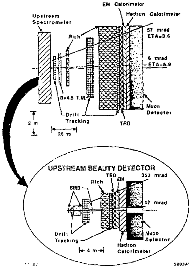
Fig. 5 B Spectrometer from the Berkeley SSC Workshop.
