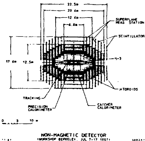
Fig. 1. Nonmagnetic Detector from the Berkeley SSC Workshop.
