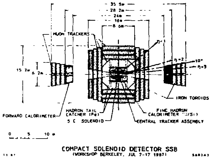
Fig. 3. Compact Solenoid Detector SSB from the Berkeley SSC Workshop.
