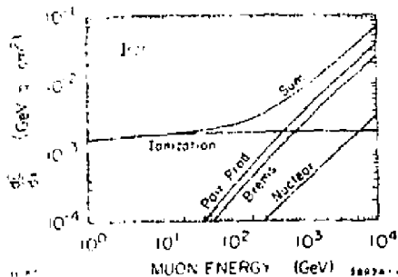
Fig. 11. Contributions to the energy loss in iron from ionization, bremsstrahlung, pair production, and nuclear interaction and their sum as functions of the muon energy. (From Reference 10.)
