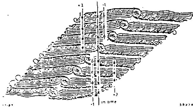
Fig. 8. Jet cell, showing electron drift lines and isochrones. Superimposed on this is a high-momentum track, together with its associated hits, and the apparent hits for a similar track from the previous bunch crossing or the one occurring three crossings later. Left-right ambiguities are omitted for clarity. (From Reference 6.)
