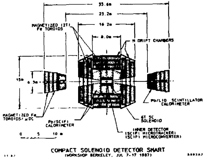
Fig. 2. Compact Solenoid Detector SMART from the Berkeley SSC Workshop.
