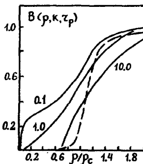
Fig.1. Function (5) at E = 1 keV (solid lines), E = 0.1 keV (dashed line). Numbers near solid lines are the values of parameter \tau_p in units of R .
