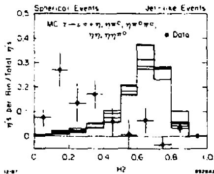
Figure 3: Distribution of the event shape parameter H2 for events with reconstructed \eta in the old inclusive analysis (points with error bars), compared to the distributions of the \eta signals in various Monte Carlo samples (histograms). The distributions are normalized to 1.
