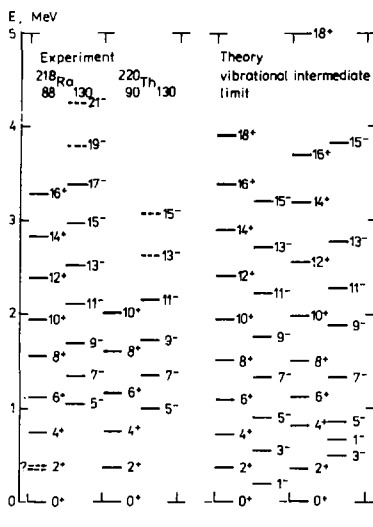
Figure 1. Reproducing the yrast line of actinide isotones with nearly vibrational spectra. Experiment from refs. /57-59/. Theory in the vibrational limit: from the first hamiltonian (3) with \xi^3 = 3\xi^1 = 540 keV, \beta_{\frac{3}{7}}^3 = 10 keV; theory in the intermediate limit: from the third, fourth or fifth hamiltonian (3) with \beta_{\frac{1}{5}}^1 = 118 keV, \beta_{\frac{1}{3}}^1 = -18.5 keV; all other parameters equal to 0.
