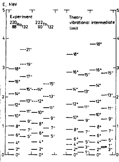
Figure 2. Reproducing the yrast line of actinide isotones with nearly transitional spectra. Experiment from refs. /59-61/.
