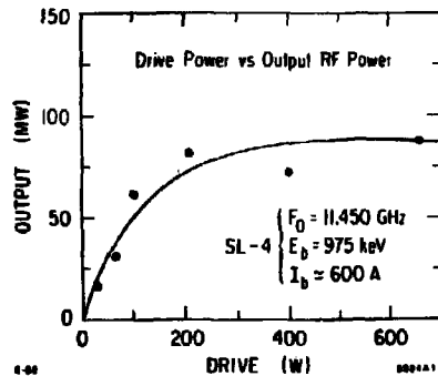
Fig. 12. Drive power versus output power of SL-4.
