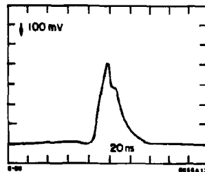
Fig. 11. Output power pulse of SL-4.
