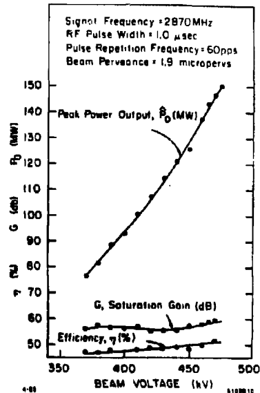
Fig. 3. Measured characteristics of experimental 150 MW klystron.
