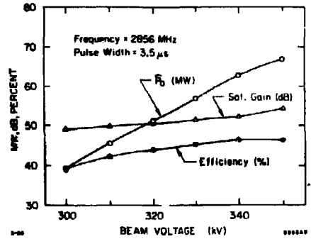
Fig. 1. Typical characteristics of production SLC klystron.
