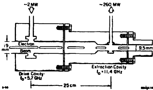
Fig. 8. Schematic of subharmonic drive experiment, SHARK.
