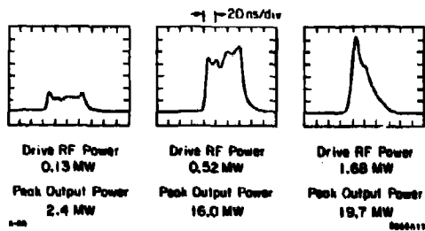
Fig. 9. SHARK RF output pulse shape for various drive powers.
