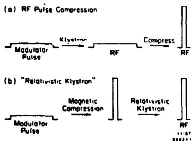
Fig. 5. a) Illustration of RF pulse compression. b) Illustration of magnetic compression.
