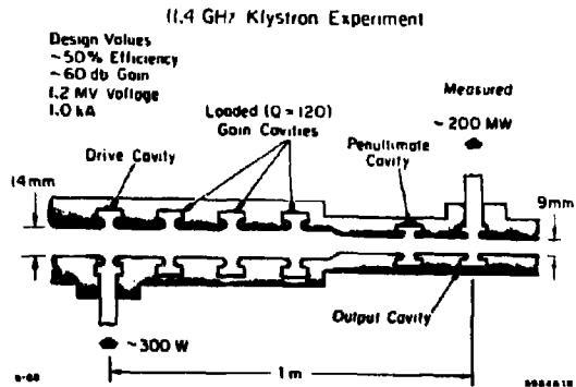
Fig. 10. Schematic of relativistic klystron, SL-4.
