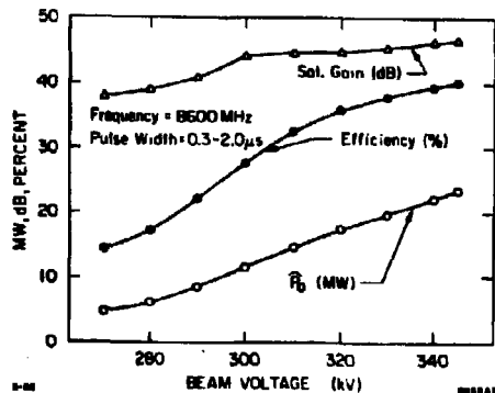
Fig. 4. Measured characteristics of experimental X-band klystron.
