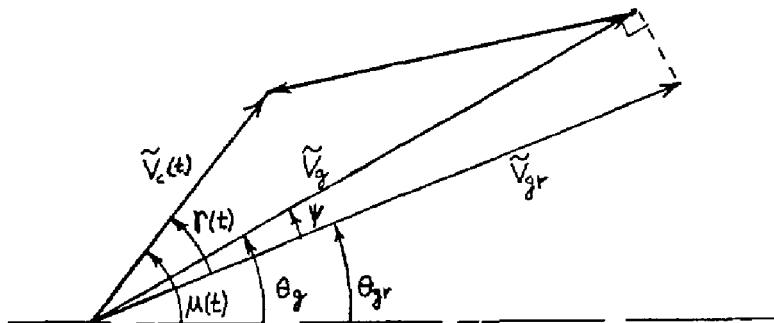
Fig. C-1 -- Diagram showing phase angles used to compute angle \gamma(t) between \tilde{V}_c(t) and \tilde{V}_{gr} .
