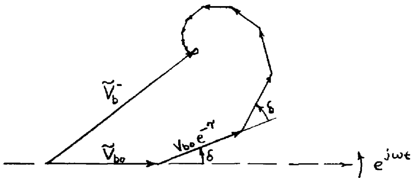
Fig. 5 -- Diagram illustrating the multiple-pass build-up of a beam-induced voltage in a cavity.
