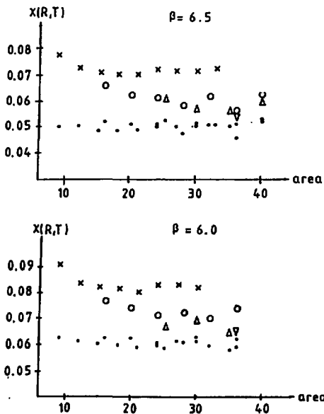
Fig. 8. The Creutz ratios for different areas and two values of \beta = 4/g^2 . The black dots represent the Creutz ratios corrected for string vibrations, x corresponds to \chi(3, T) ; o corresponds to \chi(4, T) ; \Delta corresponds to \chi(5, T) ; \nabla corresponds to \chi(6, T)
