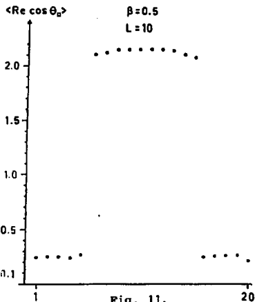
Fig. 11. Picture of the QED string in 2 dimensions. The charges are separated 10 lattice units
