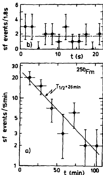
Fig. 2. Time distributions of spontaneous fission events recorded in the reaction ^{249}\text{Cf} + ^4\text{He} at t_{\text{lab}} = 32.4 MeV by using the "tape recorder" system: (a) the distribution obtained in detecting the ground-state spontaneous fission of ^{250}\text{Fm} ; (b) the distribution obtained in searching for a spontaneous fission branch in the decay of the 1.8-s K isomer ^{250m}\text{Fm} .
