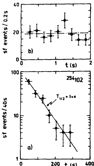
Fig. 3. Time distributions of spontaneous fission events recorded in the ^{208}\text{Pb} + ^{48}\text{Ca} reaction: (a) the distribution obtained in detecting the ground-state spontaneous fission of ^{254}\text{102} (the net result of bombardments 5 and 6); (b) the distribution obtained in searching for a spontaneous fission branch in the decay of the 0.28-s K isomer ^{254\text{m}}\text{102} (the net result of bombardments 7 and 8). See also Table III.
