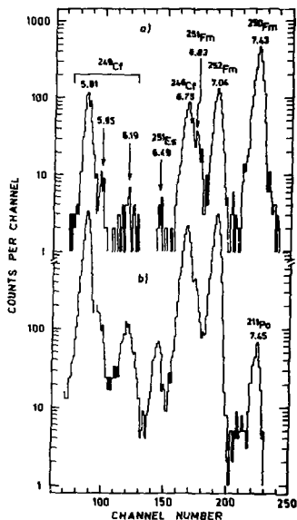
Fig. 1. Alpha-particle-energy spectra from radioactivities produced in reactions of 32.4-MeV ^4\text{He} projectiles with ^{249}\text{Cf} . The spectra were recorded in the time intervals 90-110 min (a) and 14.0-25.1 h (b) following bombardment.
