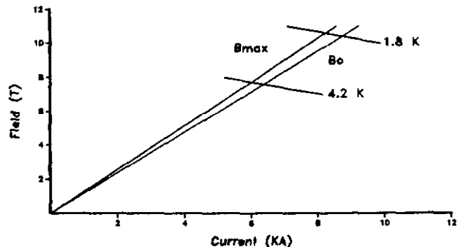
Figure 1. Load line and conductor characteristics.
