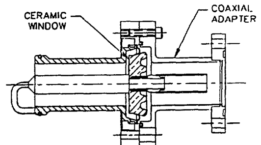
Fig. 4 Power Window
