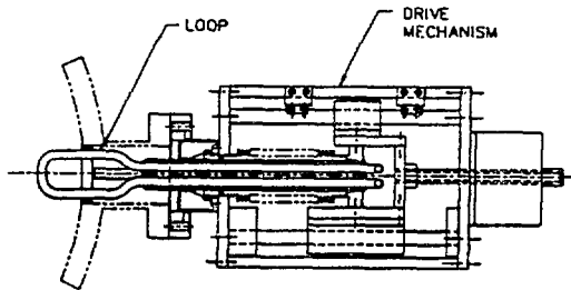
Fig. 3 Motor Driven Operational Tuner
