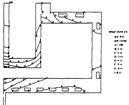
Fig. 2 Temperature Contours in the RF Cavity
