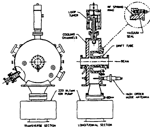
Fig. 1 RF Cavity Assembly
