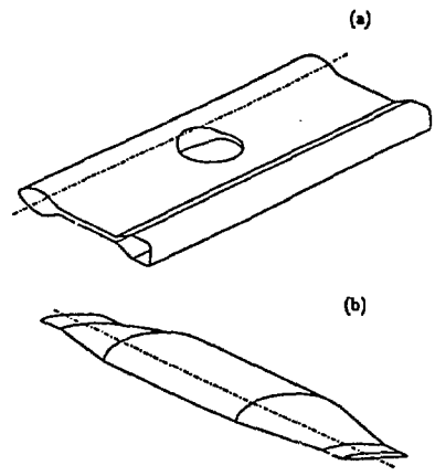
Fig. 1. Examples of the geometries studied in the computer simulations: (a) A beam chamber with an antechamber and a crotch absorber. (b) A transition between the chamber and the ID section, both of an elliptic cross section (one half of the structure).
