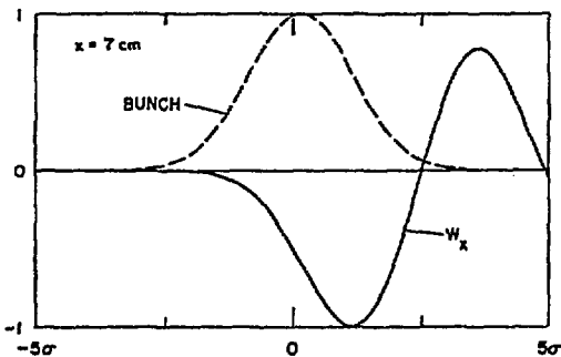
Fig. 5. An example of a negative first peak of the horizontal wake potential.
