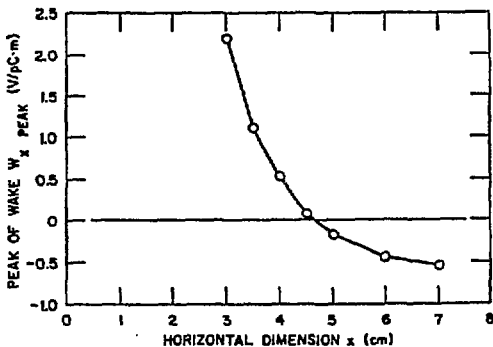
Fig. 4. A smooth transition from positiveness to negativeness of the first peak of the horizontal wake potential.
