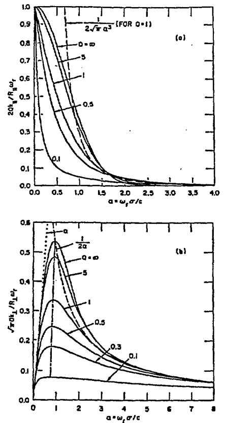
Fig. 8. Loss factors as a function of bunch lengths for a broad band resonator in normalized units: (a) longitudinal. (b) transverse.
