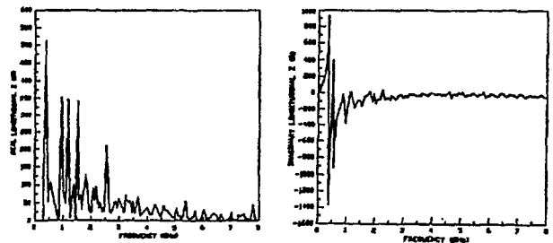
Fig. 6. Examples of the wake potentials and the impedance spectra (for an RF cavity).
