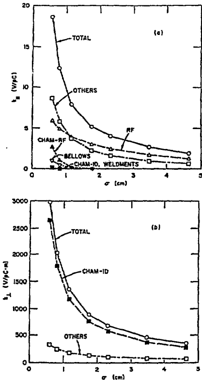
Fig. 7. Examples of the k(\sigma) curves: (a) longitudinal. (b) transverse.
