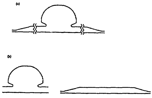
Fig. 2. (a) A complex structure, consisting of an RF cavity and two tapered parts, is decomposed to three components. (b) These components are then recomposed to form two new structures. Both (a) and (b) give the same impedance, while (b) is easy to compute.
