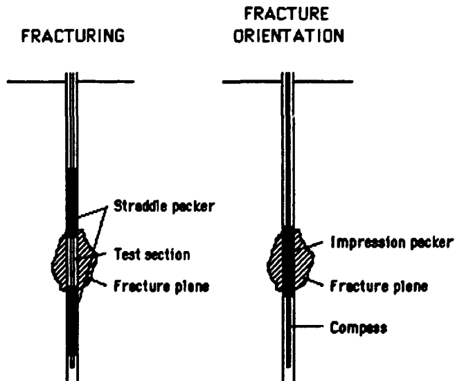
Figure 2-3. Packer configuration in the borehole during testing.
