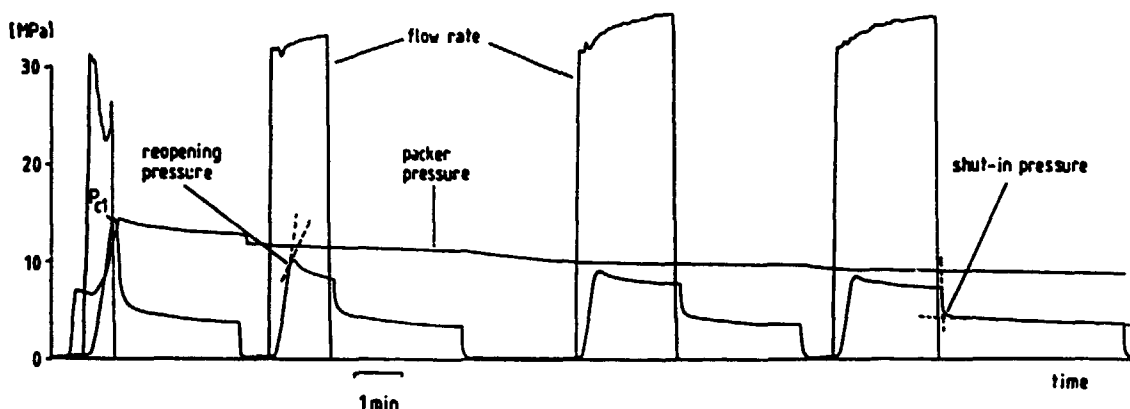
Figure 2-2. A typical hydrofracturing field record for crystalline rocks in Sweden. Getinge, Southern Sweden, 205.1 m depth.
