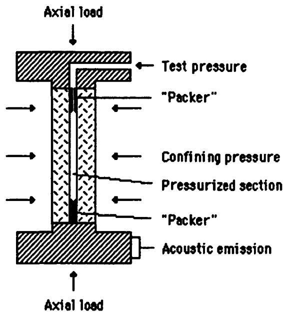
Figure 2-1. Laboratory simulation of hydraulic fracturing for determination of the tensile strength of the rock.
