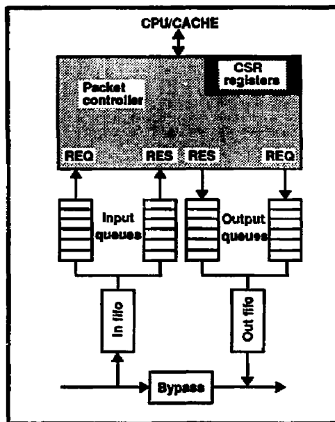
Figure 9. Node interface.
