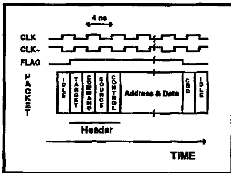
Figure 6. Packet format.
