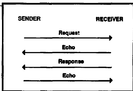
Figure 8. Split transaction handshake.
