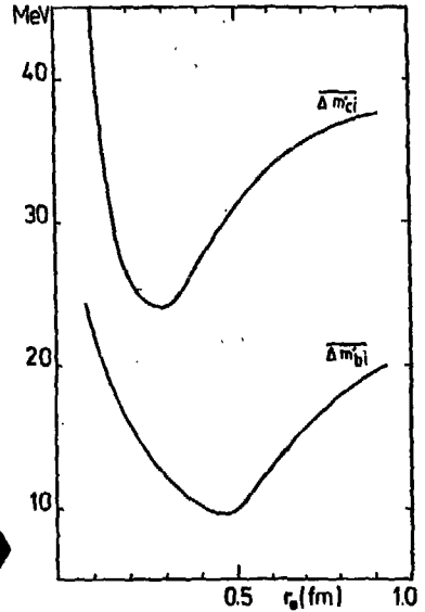
Fig. 3. The mean square errors of m'_{bi} and m'_{ci} as functions of r_0 .
