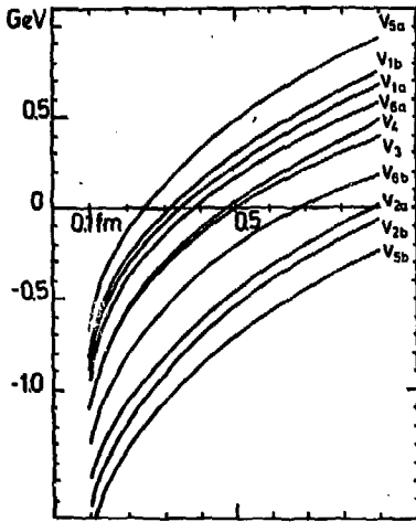
Fig.1. The underlying potentials in the region 0.1 < r < 1.0 fm.
