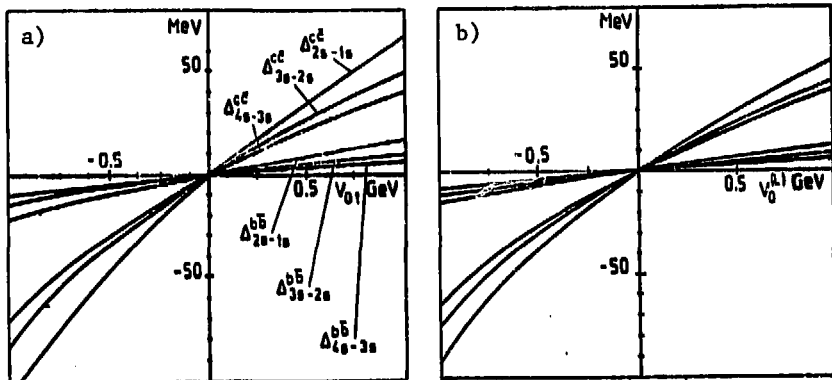
Fig. 4. a) The change of the three lowest S level spacings for c\bar{c} and b\bar{b} as function of V_{01} in the Cornell potential model with k = 0.47 and a = 0.19 \text{ GeV}^2 . b) The same functions as in Fig. 4a for a pure linearly raising potential V^{(L)}(r) = ar .
