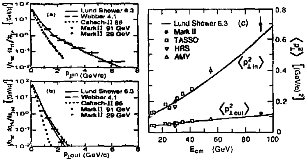
Fig. 2. Corrected charged-particle distributions (a) 1/\sigma_{had} d\sigma_{trk}/dp_{Lin} and (b) 1/\sigma_{had} d\sigma_{trk}/dp_{Lout} compared with the predictions of several models and with Mark II data at 29 GeV. (c) Comparison between means of p_{Lout}^2 and p_{Lin}^2 distributions for e^+e^- experiments at various E_{cm} .
