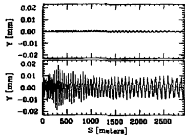
Figure 2: Difference orbit after correction in the NLC.
