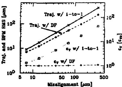
Figure 6: 1-to-1 and DF correction vs. the misalignments.
