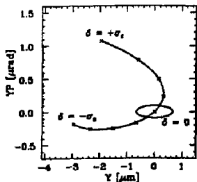
Figure 3: Y-Y' phase-space at the end of the NLC after 1-to-1 correction.
