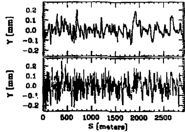
Figure 1: Trajectory after correction in the NLC.
