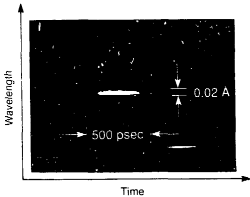
Figure 4-14. A schematic diagram of a high-resolution streak spectrograph for time-resolved measurements of x-ray-laser line widths. This instrument was recently installed on the two-beam Nova chamber for joint experiments with LLNL. The streak-camera image shows the 206-Å laser line from a 4-cm-long x-ray laser using neon-like selenium. Sub-Doppler line narrowing, as observed here, is a characteristic of lasing.
