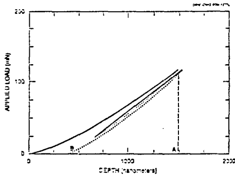
Figure 1. Loading curve for fiber remaining intact.
