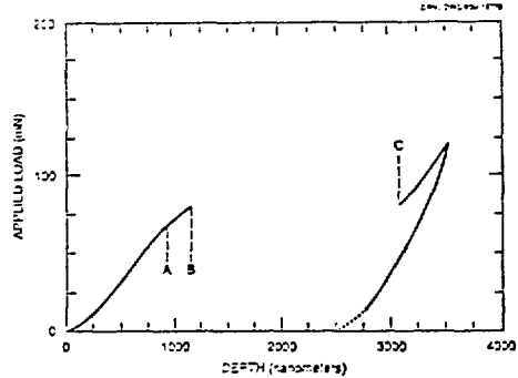
Figure 2. Loading curve for fiber debonding and push-out.
