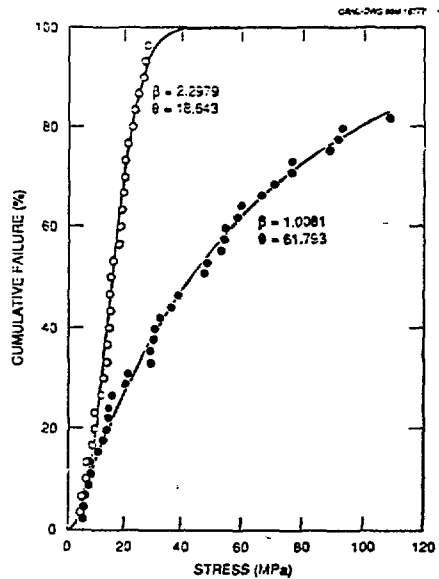
Figure 5. Cumulative Weibull Distribution of data.
