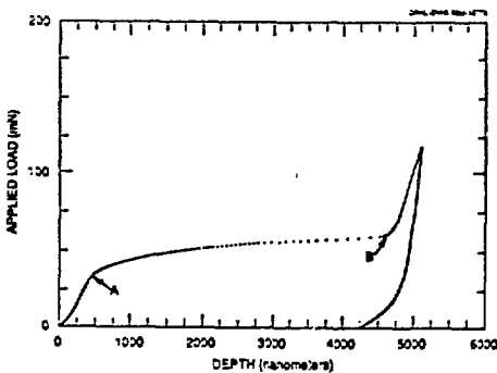
Figure 3. Loading curve for frictional sliding
