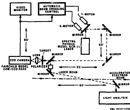
Fig. 1. Compton polarimeter experiment block diagram.
