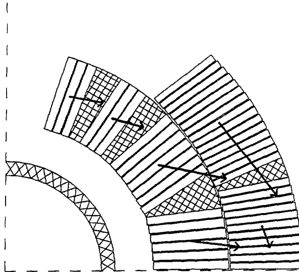
Figure 8: Lorentz Force on each block.
