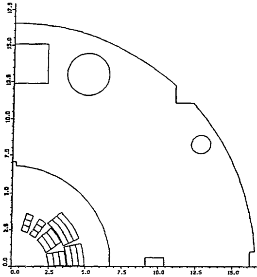
Figure 4: POISSON model for SSC 50 mm Dipole.
