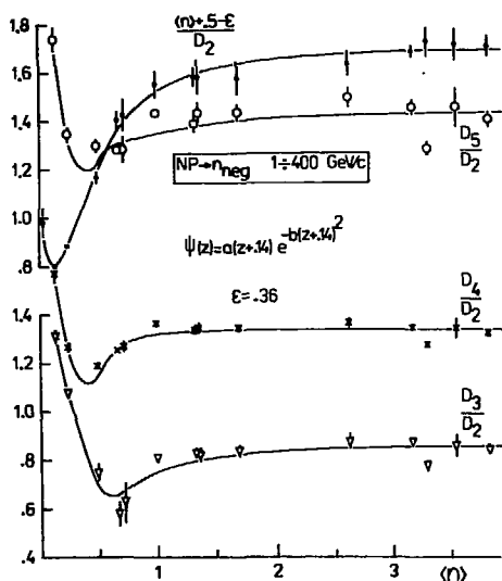
Fig. 4. Ratios which should go fastly to the plateau with increasing energy (according to (12)). The curves are obtained by eqs. (4)-(6) with \Psi(z) presented in the figure. The coefficients a and b calculated from (2) are equal to 1.251 and .618, respectively.
