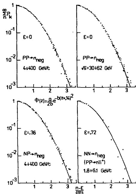
Fig.3. Dependence of the integral probability \sum_{k=0}^{\infty} P_k on (n-\epsilon)/\langle m \rangle for various nucleon-nucleon reactions (see (15)-(18)).
