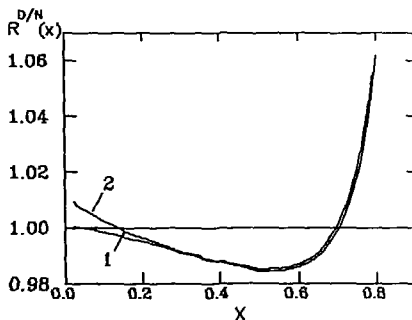
Fig.2. Ratio of the structure functions of the deuteron and free nucleon ( 1- impulse approximation 2- IA + MEC contribution ).
