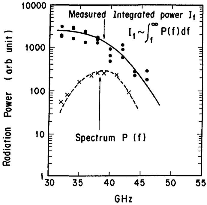
Fig.7 Spectrum of super radiation.
