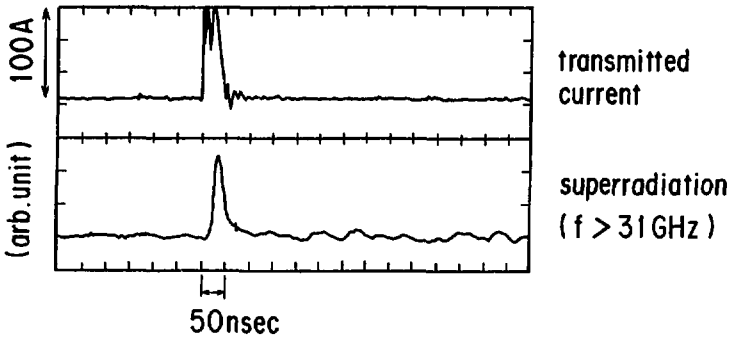
Fig.6 Wave form of the super radiation.
