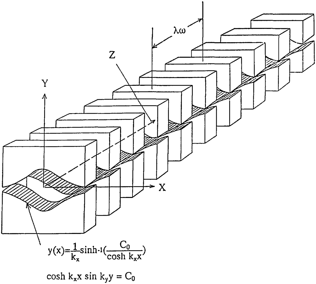
Fig.1 Focusing Wiggler and coordinate system.
