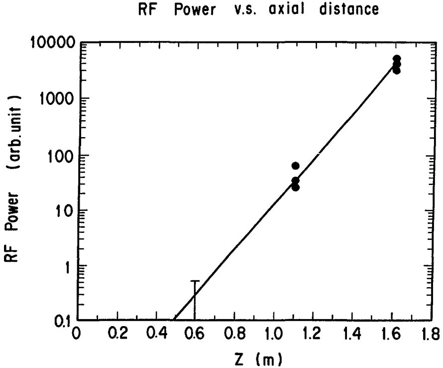
Fig.8 Relation between radiation power and integration length.
