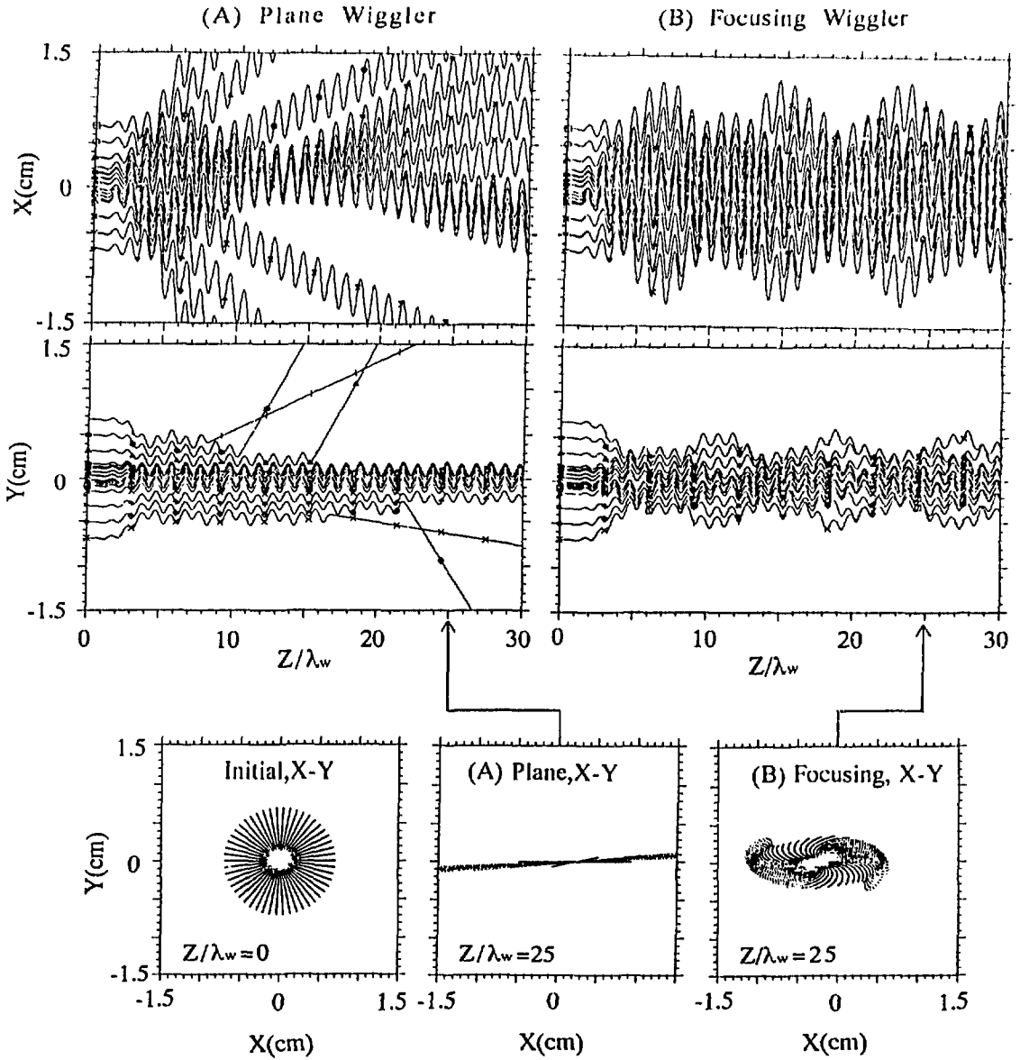
Fig.2 Beam trajectories in the case of both planes and focusing wiggler.
