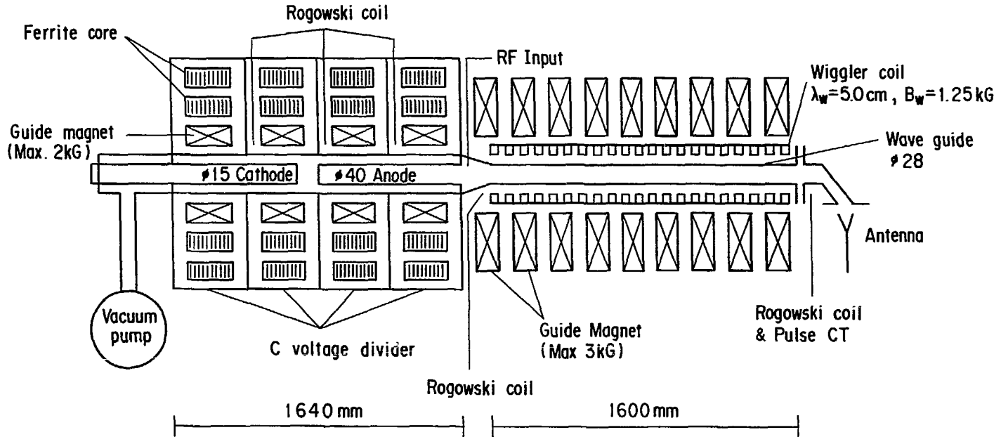
Fig.3 Schematics of the experimental apparatus.
