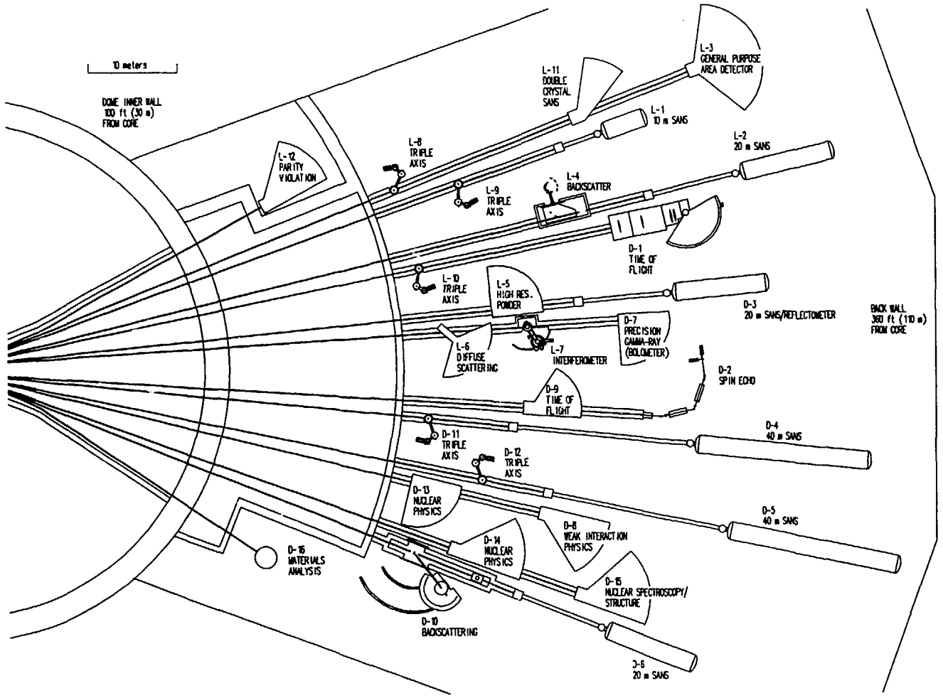
Figure 5. The Cold Neutron Guide Hall.
