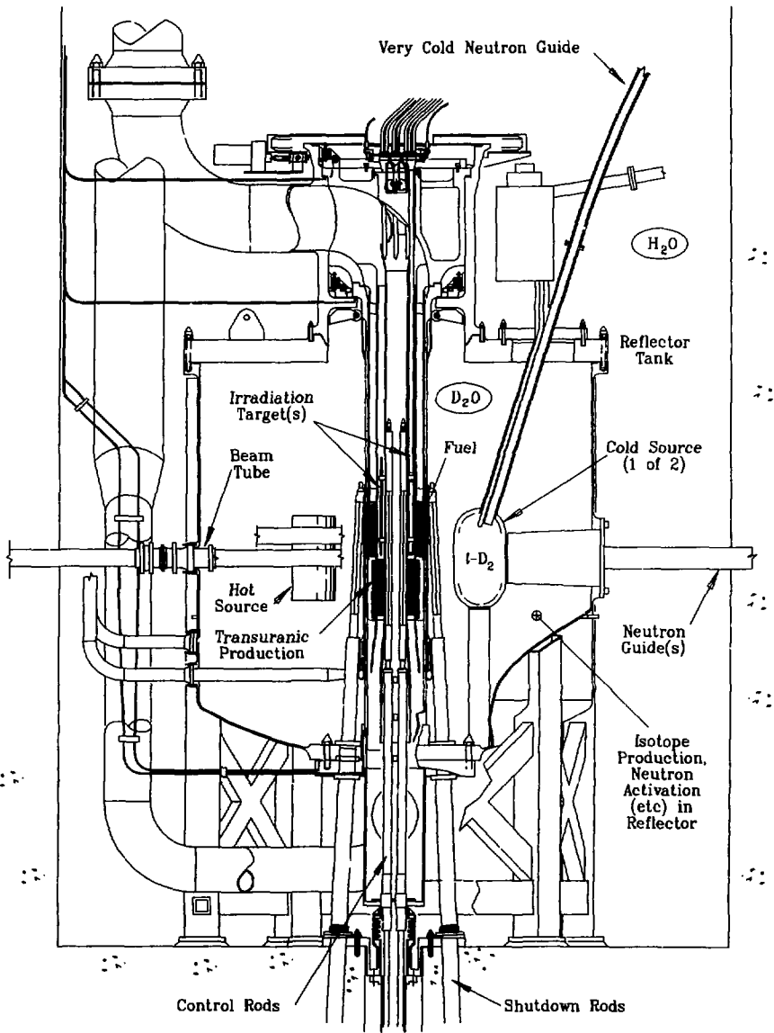
Figure 2. The ANS reactor assembly.
