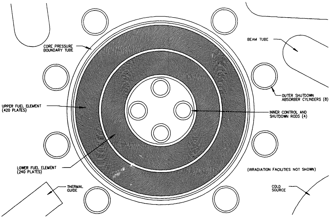
Figure 1. Plan view of the ANS reactor core.
