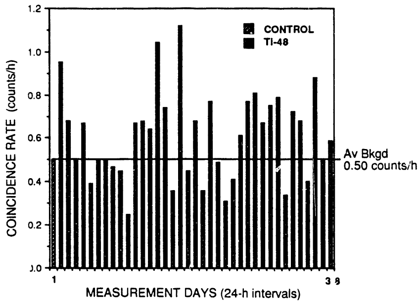
Fig. 5. Neutron coincidence results for sample Ti-48 in detector system 2. Each data interval corresponds to the average rate for ~24 h of counting. Most of the time intervals were initiated with an LN temperature cycle.
