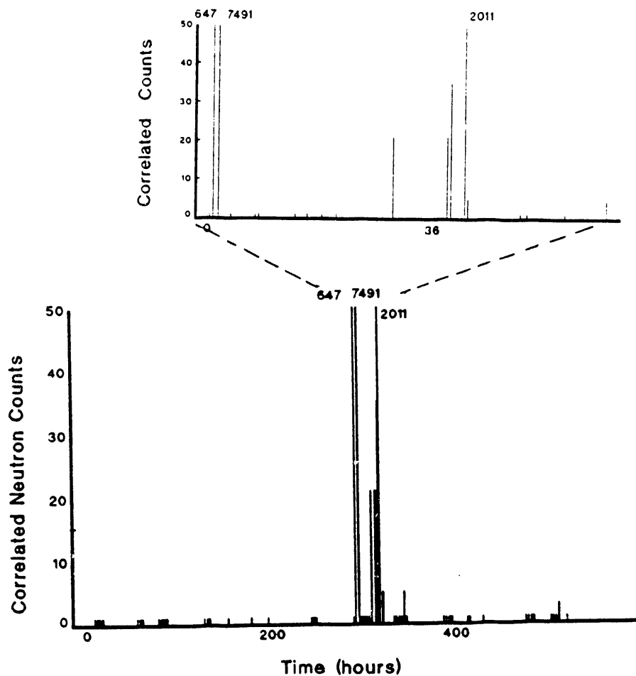
Fig. 3. Neutron coincidence results for sample DD-17 in detector system 1 where the counting intervals are 100 s. The top graph shows a time expansion of the active period. The 280 h of data prior to the active period correspond to the control sample or alternatively an inactive sample (DH-13) in the detector including LN temperature cycles.
