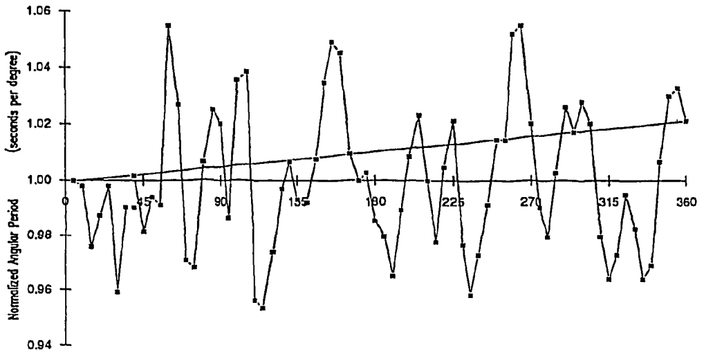
Fig. 6 Normalized Angular Period (seconds per degree, the average being 2.072 secs per degree) vs toroidal angle of the calibration train
