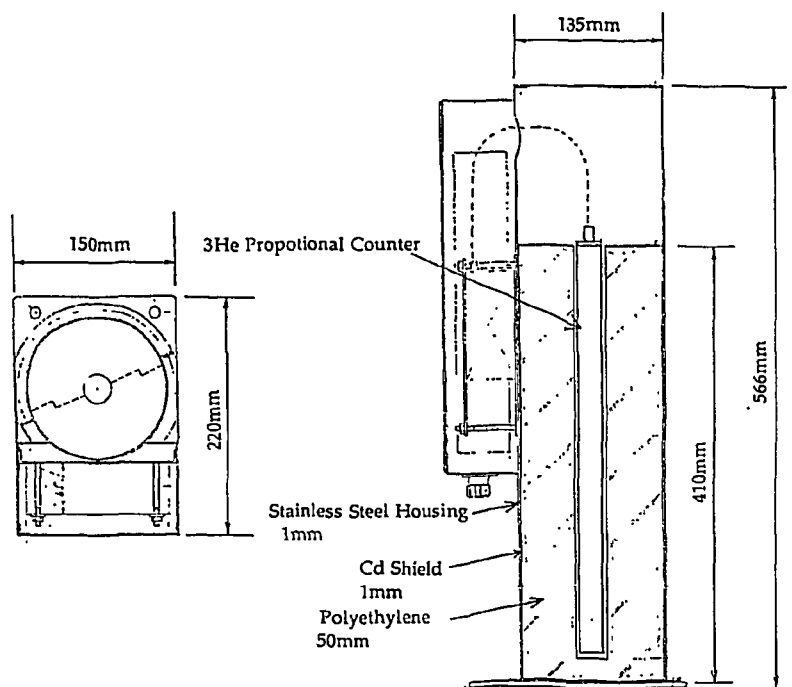
Fig. 3 Schematics of the ^3\text{He} proportional counter
