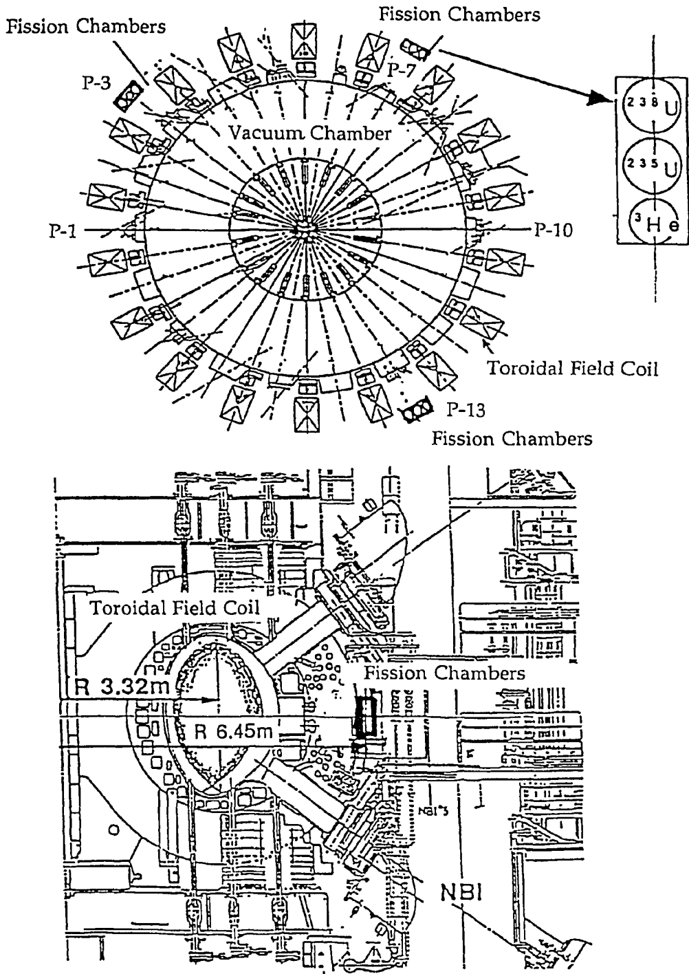
Fig. 1 Arrangement of the neutron detectors on the JT-60 Upgrade
