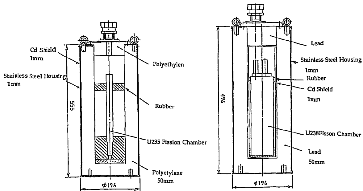
Fig. 2 Schematics of the ^{235}\text{U} and ^{238}\text{U} detectors
