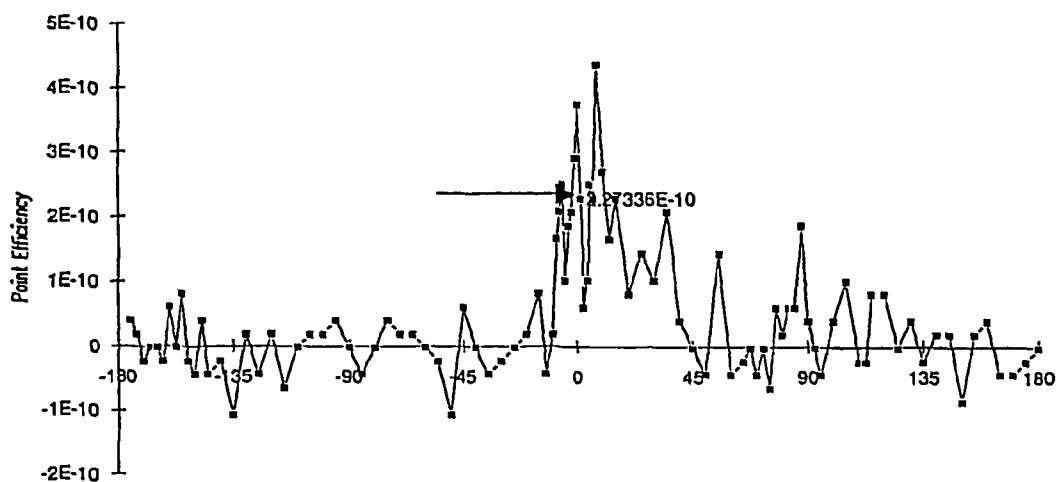
Fig. 14 ^{238}\text{U} point efficiency, calculated by subtracting a background of 154 counts per 1000 seconds, vs toroidal angle. The arrow and value label a single data point taken for 10000 seconds
