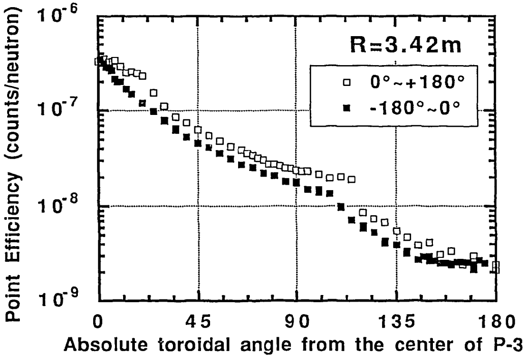
Fig. 12 ^{235}\text{U} point efficiency vs absolute value of the toroidal angle
