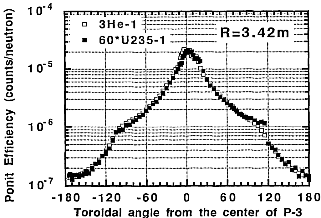
Fig. 10 Point Efficiency (log scale) vs toroidal angle for two detectors in Bay P-3. The data for the ^{235}\text{U} detector have been multiplied by 60
