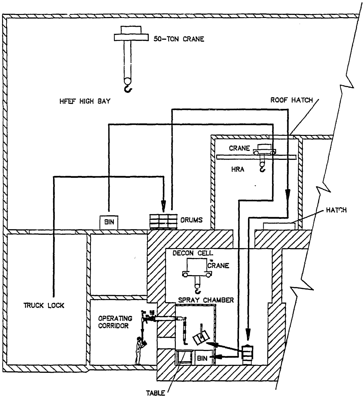
FIGURE 1 WIPP PROJECT WASTE FLOWPATHS THROUGH HFEF
