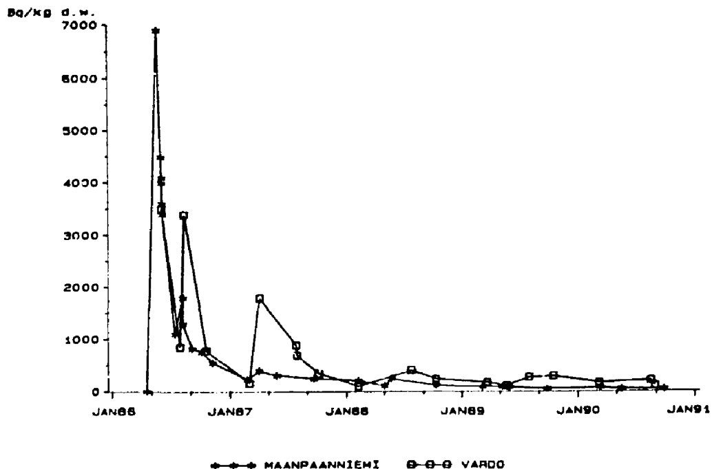
Fig.2. Concentrations of 137 Cs in sewage sludge at Rauma (Maanpäänniemi) and at Loviisa (Vårdö) in 1986-1990.
