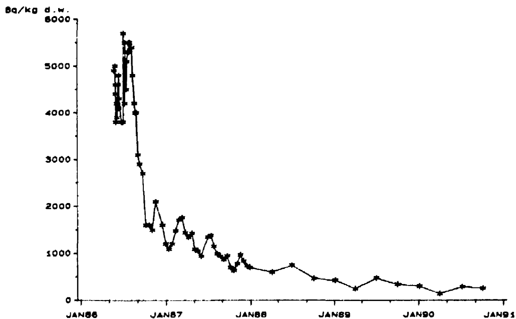
Fig.3. Concentrations of 137 Cs in sewage sludge at Helsinki (Kyläsaari) in 1986-1990.
