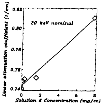
Fig. 4. Least-square fit of the measured attenuation coefficients in the 20-keV image (Fig. 2) as a function of the KOH concentration in the holes.
