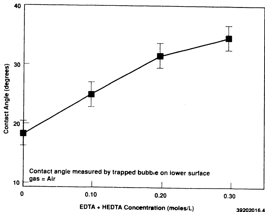
FIGURE 10. Contact Angle on Sapphire Versus Complexant Concentration in Synthetic Waste
