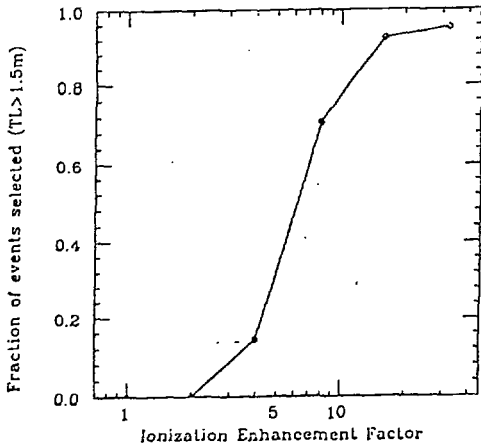
Figure 2. Fraction of fake monopoles passing ionization cut vs. enhancement.
