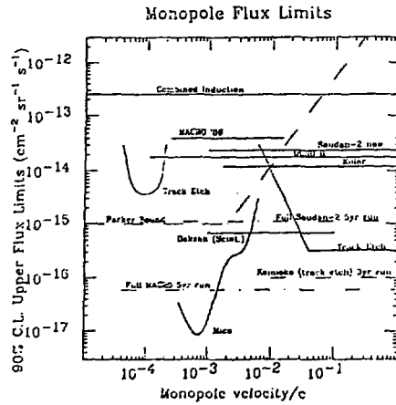
Figure 3. Recent monopole flux limits.
