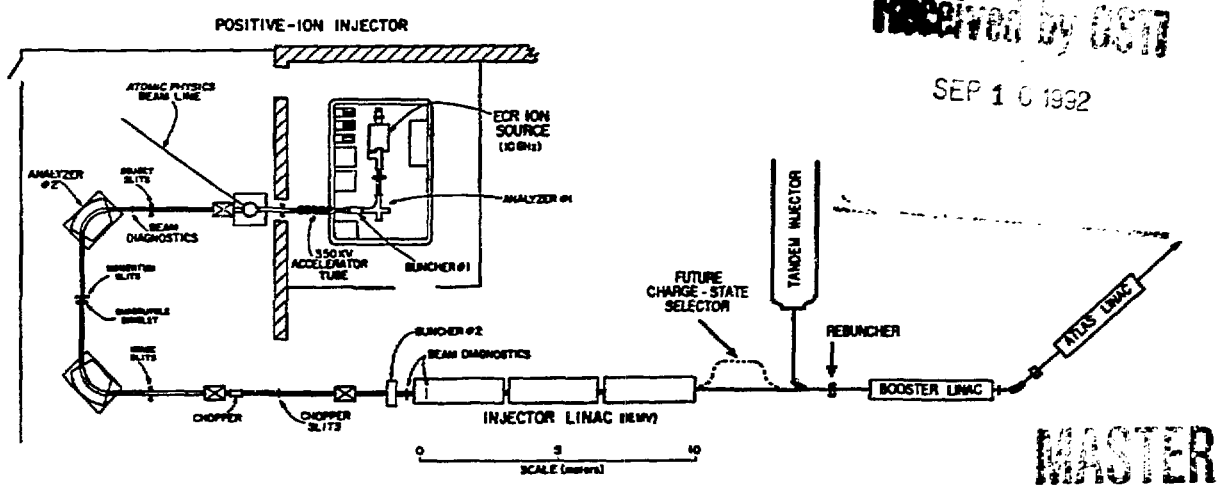
Fig. 1. Schematic floor plan of the ATLAS facility. The new PII is shown to scale with the remainder of the facility compressed and not to scale.
