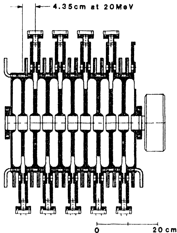
Fig. 1 A 5\beta\lambda long CCL accelerator tank at 20 MeV and 700 MHz showing close end wall spacing and fabrication complexities.
