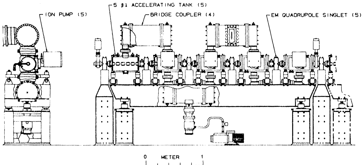
Fig. 2 5 tank 20-22.9 MeV, 700-MHz bridge-coupled DTL module.
