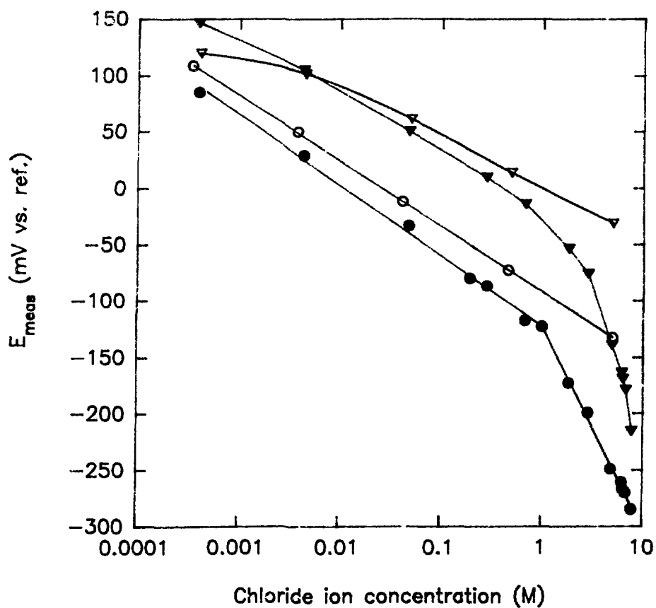
Fig. 2. Calibration curves for sodium chloride and hydrochloric acid with the solid-state and membrane-type CLISEs. Solid-state CLISE: (○) sodium chloride, (●) hydrochloric acid. Membrane CLISE: (▽) sodium chloride, (▼) hydrochloric acid.
