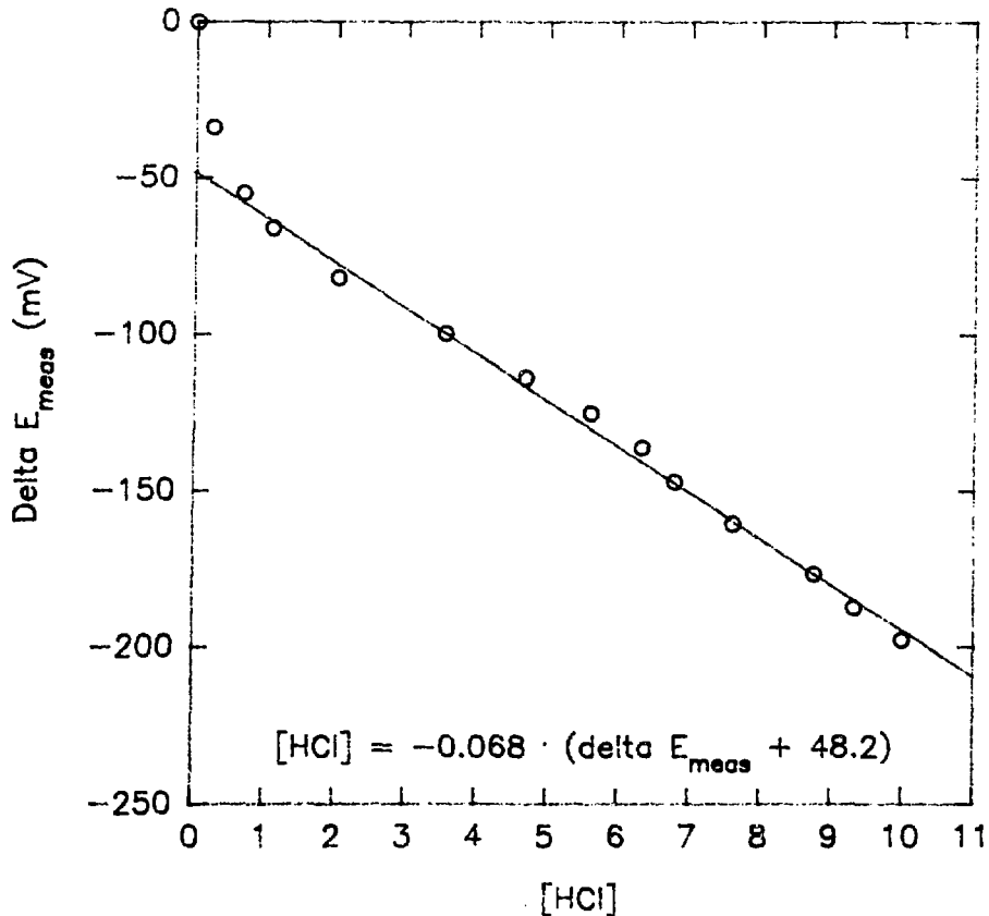
Fig. 4. Measured potential versus linear acid concentration plot for a sodium chloride/potassium chloride/hydrochloric acid system.
