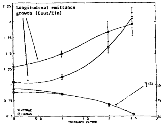
Fig. 2 Comparison DYNAC-LORAS
