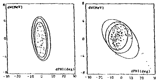
Fig. 3 Scatter plots Nominal (left), 2 tolerances (right)
