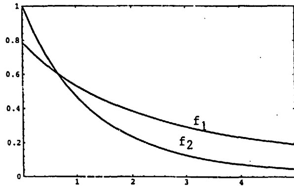
Figure 4: Auxiliary functions f_1(x) and f_2(x) .
