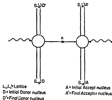
Figure 1: Two-step virtual neutron transfer reaction from a donor nucleus to an acceptor nucleus.
