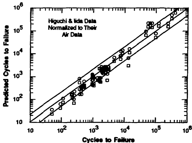
Figure 2. Comparison of Predicted and Observed Lives in Tests of Higuchi and Iida Using Air Data for Their Heat as the Reference Curve.
