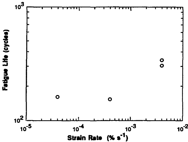
Figure 3. Fatigue Life in Water with ~0.8 ppm Dissolved Oxygen at 288°C at a Strain Range of 0.75% as a Function of Strain Rate during Rising Load Portion of Cycle
