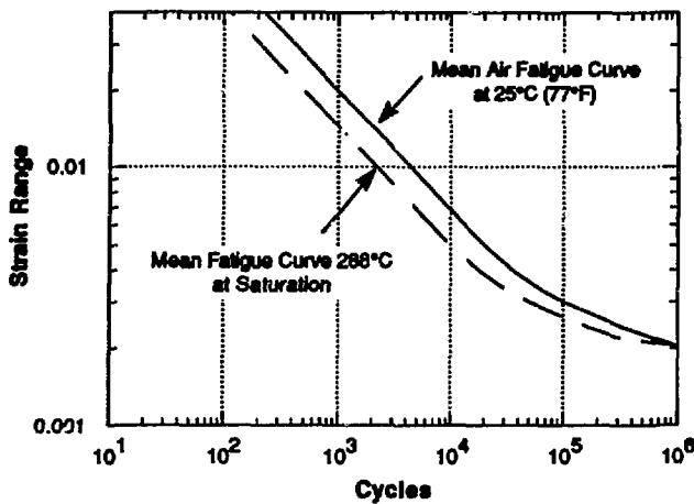
Figure 9. Proposed EAC-Adjusted Mean Fatigue Curve for Carbon Steels in Water with \leq 0.1 ppm Dissolved Oxygen.
