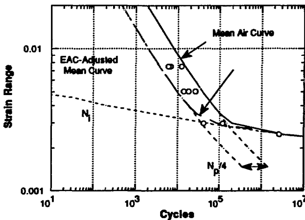
Figure 12. Proposed EAC-Adjusted Mean-Fatigue Curve for Austenitic Stainless Steels in Water at 288^\circ\text{C} with Data from Ref. 15.
