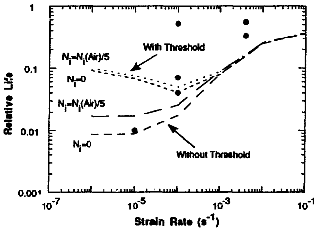
Figure 6 Comparison of Predicted and Observed Fatigue Lives of a Carbon Steel as Functions of Strain Rate for Tests Conducted at Strain Range of 0.6% in 288°C (550°F) Water Containing 8 ppm Dissolved Oxygen.
