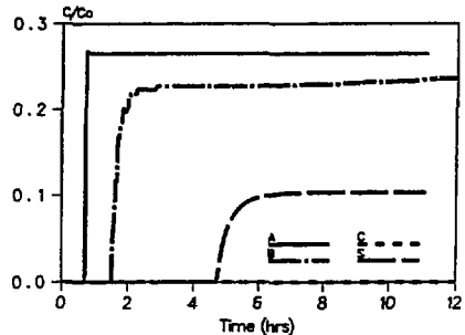
Figure 4 - Breakthrough curves for Cases A, B, C and S for radially convergent tracer tests.
