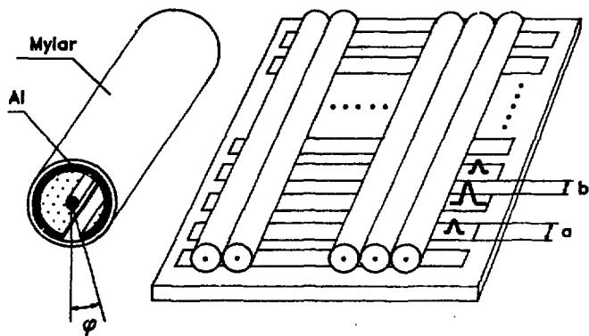
Fig.1. The scheme of the chamber (the right) and the straw (the left). Thickness of fiberglass plane is 2.5 mm. Thickness of cuprum strips is 50 \mu m. Step of strips (a) is 3, 4, 5 mm. Interval value (b) is 0.5, 0.5, 1 mm correspondingly. Diameter of maylar straw is 10 mm. Thickness of aluminized maylar is 25 \mu m.
