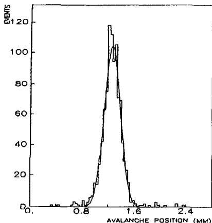
Fig.8. The detector spatial resolution for collimated X-rays beam (FWHM < 100 \mu\text{m} ).
