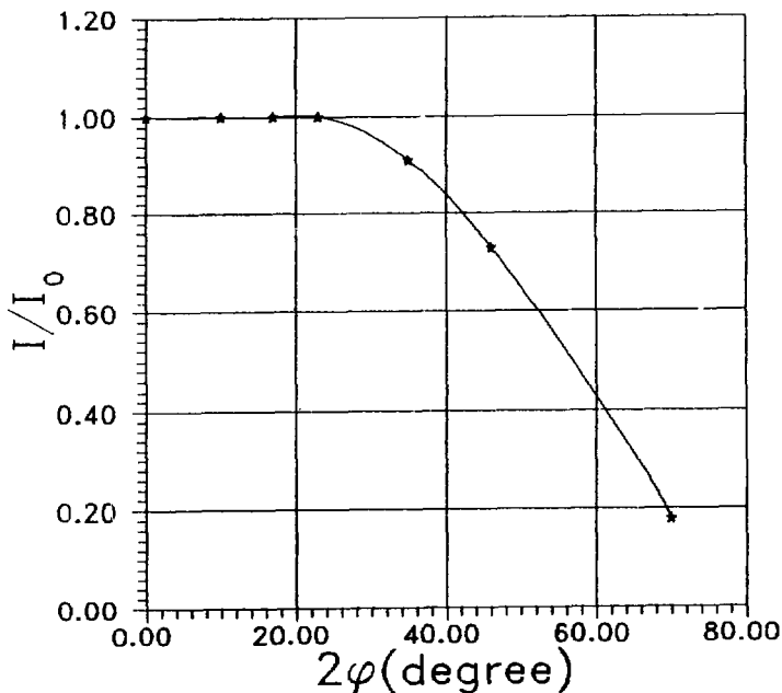
Fig.2. The straw count rate capability dependence on window angle width. The value I_0 for straws without window was 2 \cdot 10^4 l/(cm 2 sec), the diameter of X-rays beam was 1 mm. The gas gain was about 5 \cdot 10^5 , gas mixture was Ar/CH 4 (50/50).
