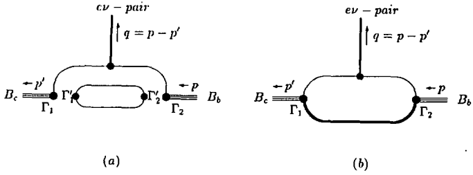
Fig.1 Heavy-Baryon Weak Form Factors in the QCM. a. Two-loop quark diagram, b. One-loop quark-diquark diagram.
