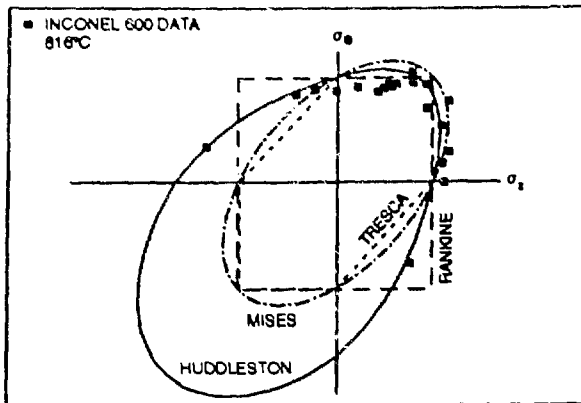
FIG. 3 BIAxIAL ISOCHRONOUS STRESS-RUPTURE CONTOUR FOR INCONEL 600
