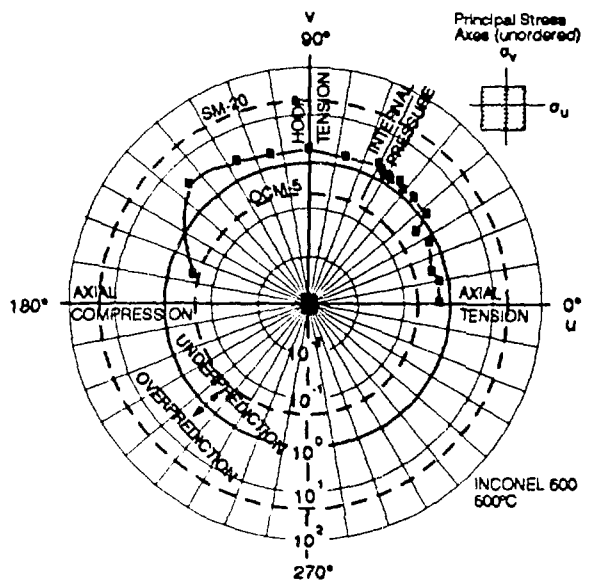
FIG. 8 CORRELATION OF THE RATIO OF PREDICTED TO OBSERVED LIFE WITH STRESS STATE BASED ON THE RANKINE THEORY
