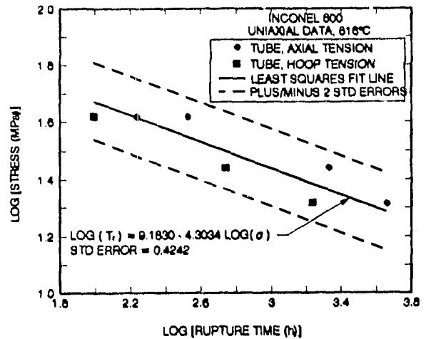
FIG. 2 BASELINE UNIAXIAL STRESS VERSUS RUPTURE TIME DATA
