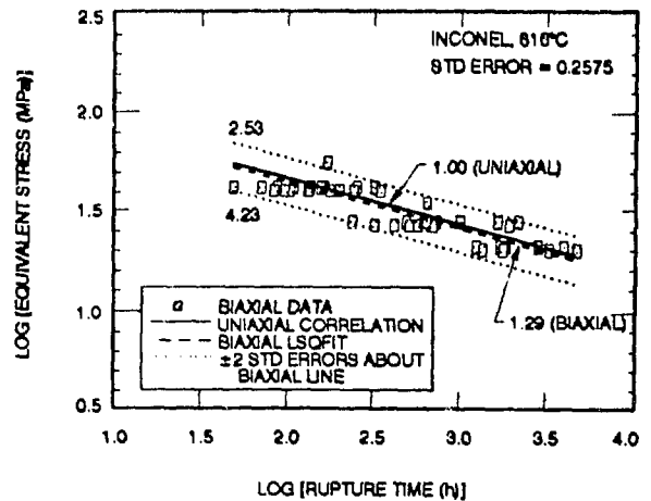
FIG. 12 MAXIMUM PRINCIPAL STRESS VERSUS BIAXIAL RUPTURE TIMES
