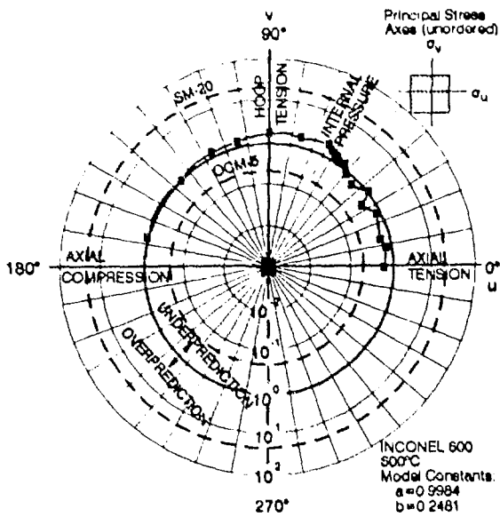
FIG. 5 CORRELATION OF THE RATIO OF PREDICTED TO OBSERVED LIFE WITH STRESS STATE BASED ON THE NEW THEORY
