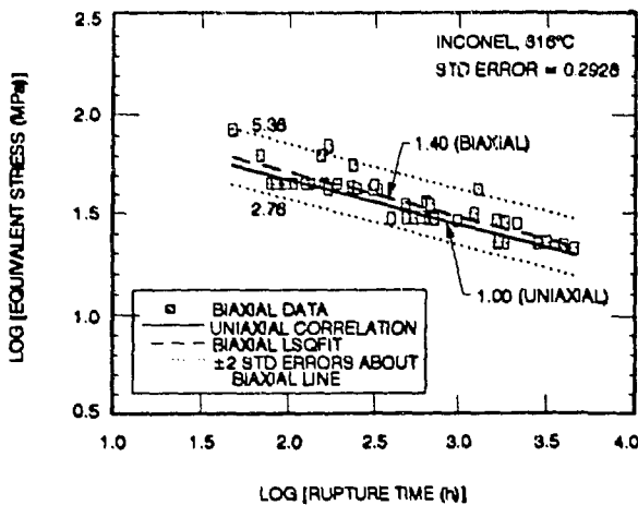
FIG. 10 TRESCA STRESS INTENSITY VERSUS BIAXIAL RUPTURE TIMES
