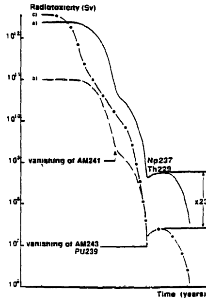
Figure 5.1 - Variation of radiotoxicity - Neptunium-237
