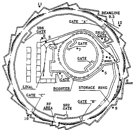
Figure 1. ALS floor plan. Pairs of neutron and gamma radiation monitors are shown as dots numbered from 1 to 12.
