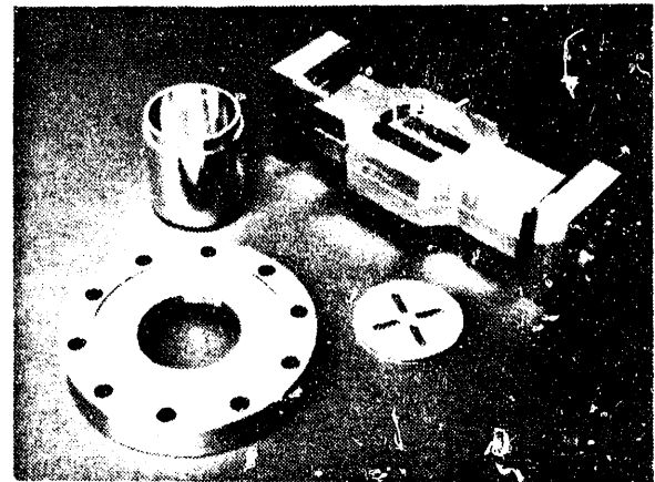
Figure 8. Transducer/combiner/divider.
