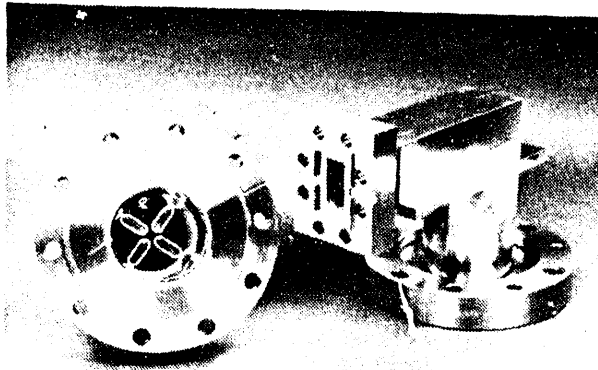
Figure 6. Completed flower-petal transducer
