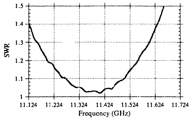
Figure 5. Transducer input VSWR
