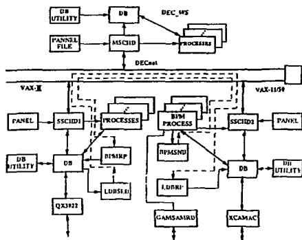
Figure 2. The upgrade of BEPC control software system
