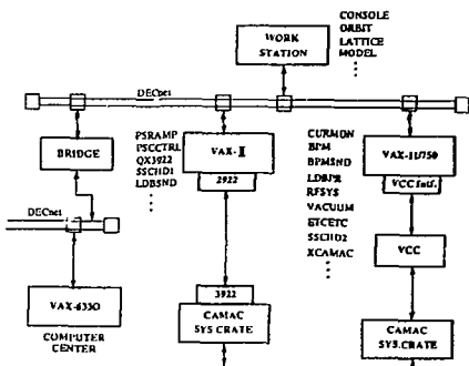
Figure 1. The upgrade of BEPC control system
